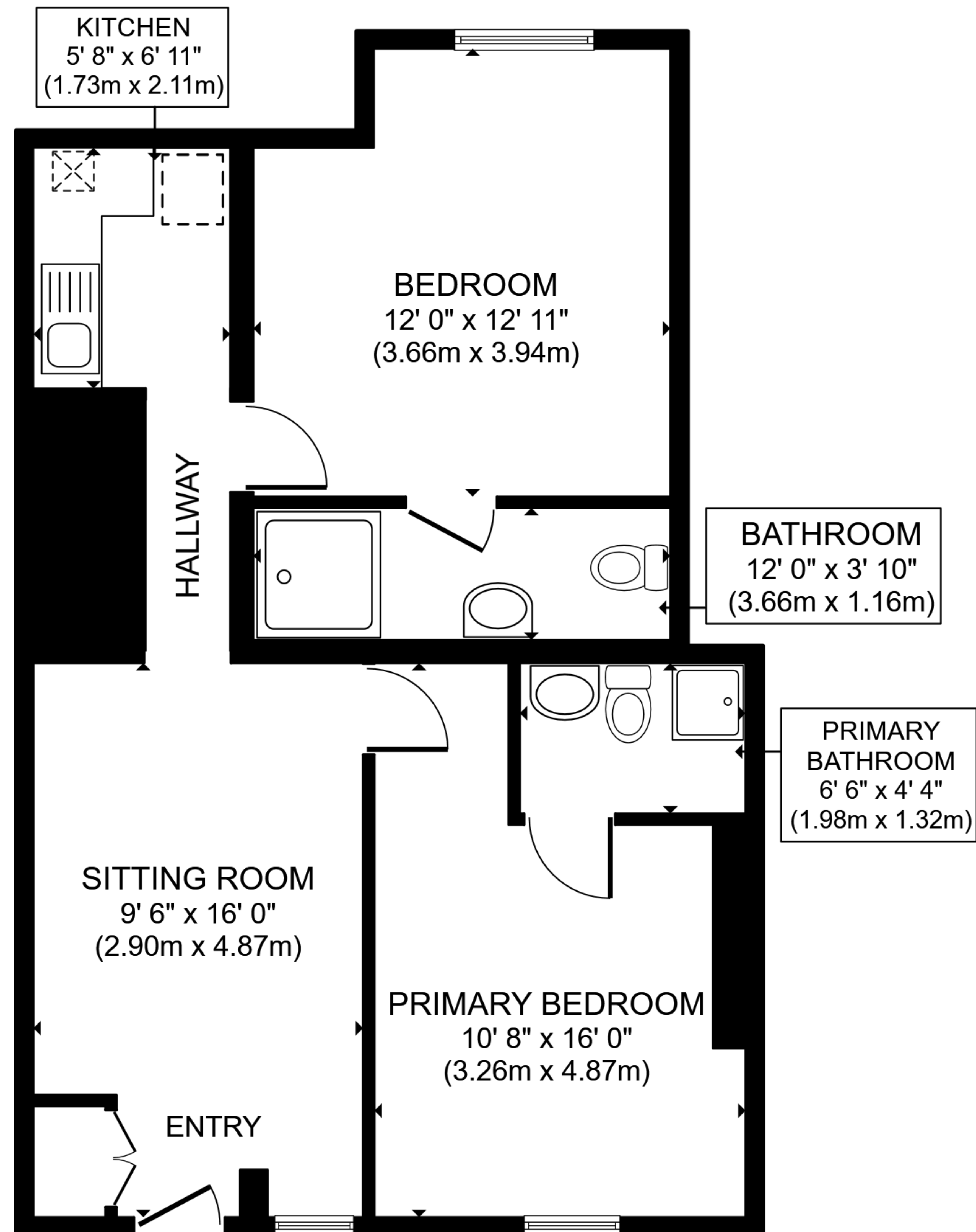
FLOOR PLAN
