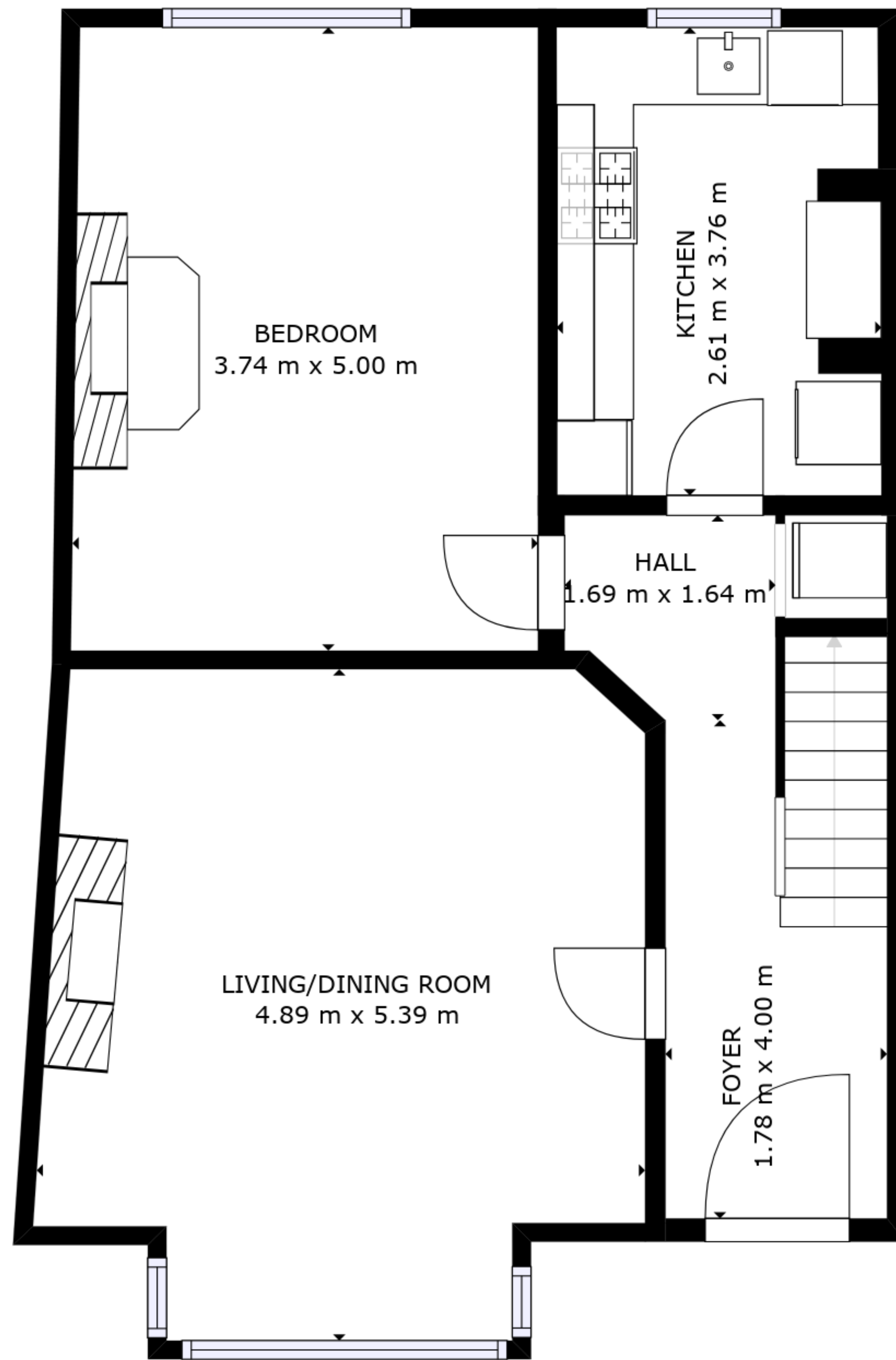
FLOOR 1
