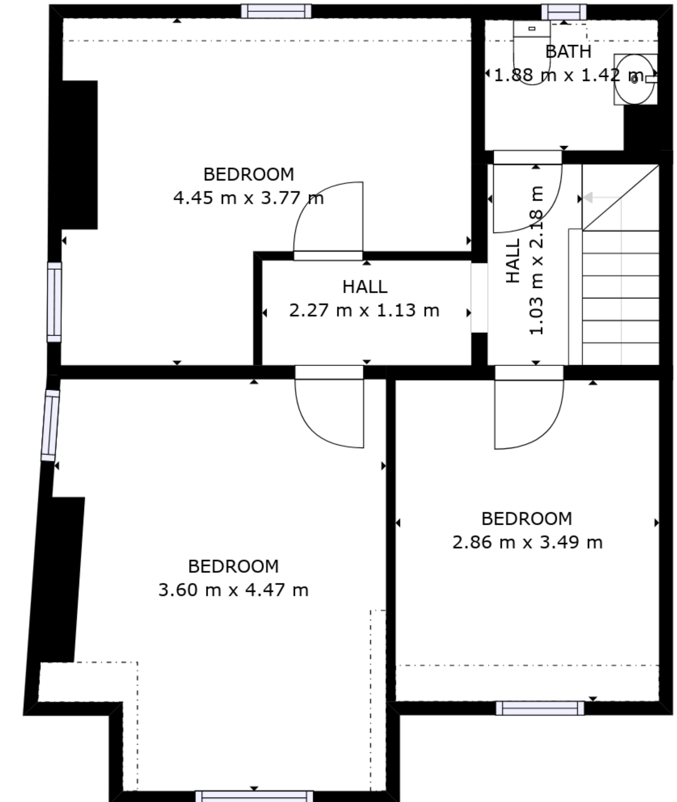
FLOOR 3
