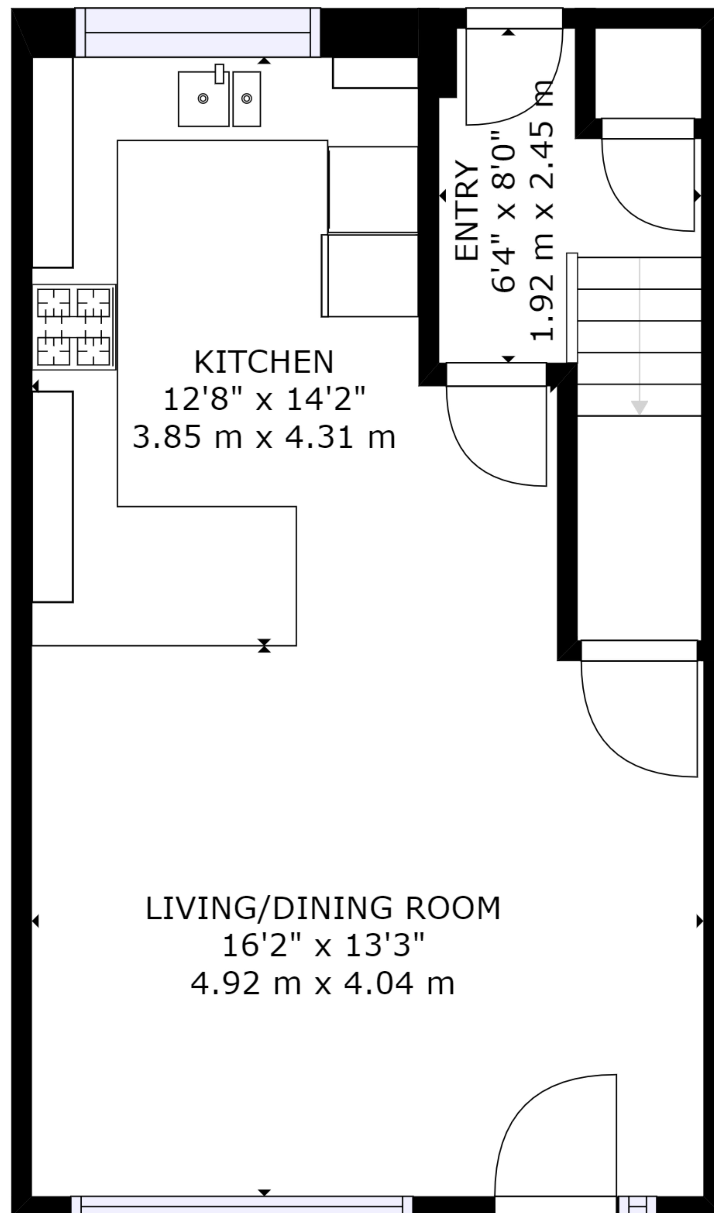
FLOOR 1
